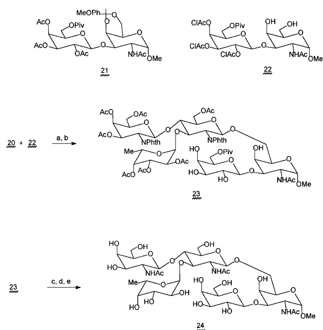
Scheme II. (a) NIS-triflic acid; \text{CH}_2\text{Cl}_2 , -65^\circ\text{C} ; (b) thiourea-lutidine, ethanol- \text{CH}_2\text{Cl}_2 (1:1, v/v), 6 h, 80^\circ\text{C} ; (c) hydrazine hydrate-methanol (4:1, v/v); (d) methanol-triethylamine-acetic anhydride (4:2:1, v/v); (e) MeOH-MeONa.
