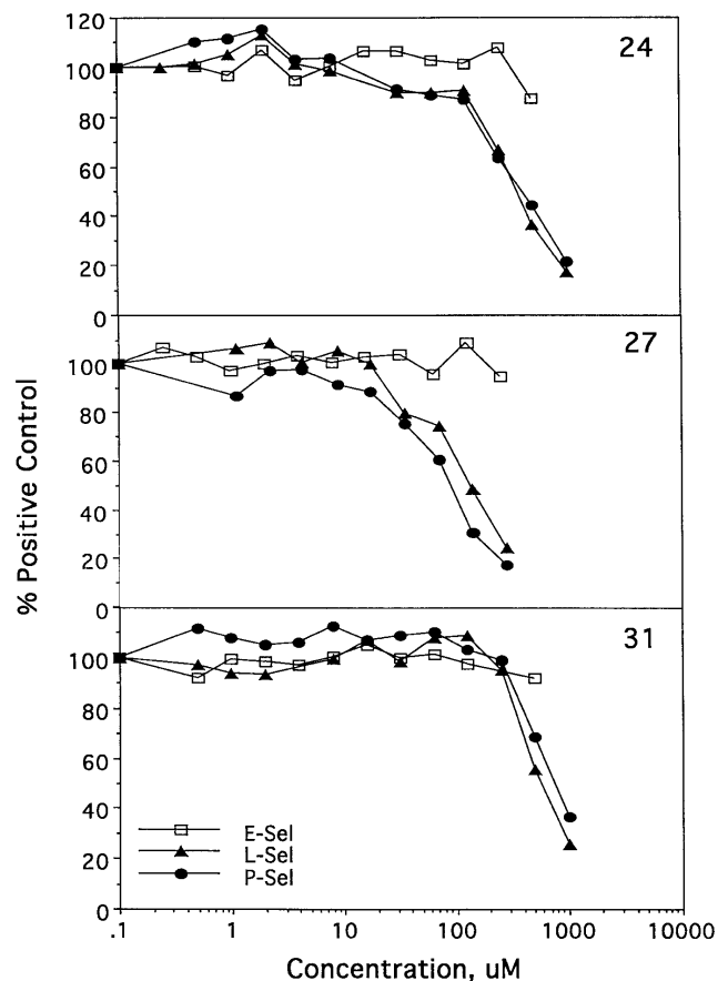
Fig. 2. Inhibitory properties of Compounds 24 , 27 , and 31 against E-, L-, and P-selectin against immobilized SLe x . Compounds 24 , 27 , and 31 were tested for their ability to inhibit the binding of each of the recombinant selectins to immobilized SLe x in ELISA inhibition experiments, as described under Materials and methods . The IC 50 values from such studies and the structures of the compounds 24 , 27 , and 31 are represented in Table III.
