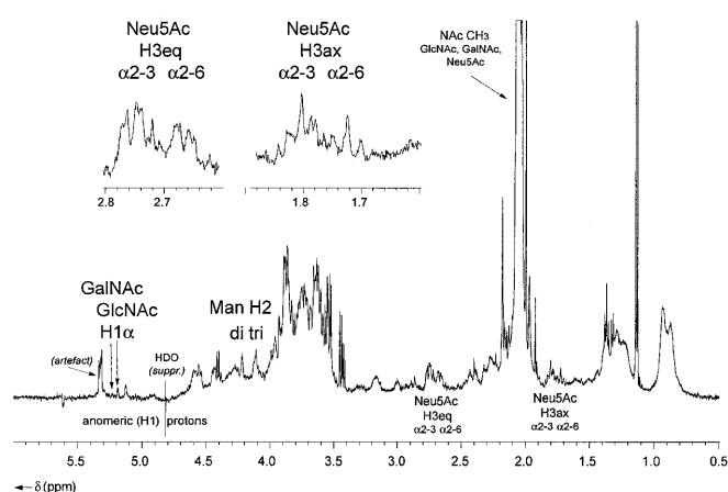
Fig. 1. ^1\text{H-NMR} spectrum of the “whole mixture” of N- and O-glycans released from bovine fetuin (2 mg) by hydrazinolysis. The spectrum was recorded at 500 MHz and 27^\circ\text{C} , in 1000 transients, using a ^1\text{H} -nanoprobe holding the sample in 40\ \mu\text{l} \text{D}_2\text{O} (pD 6.5). The HDO signal (at \delta 4.76) was selectively suppressed by presaturation. Monosaccharide and Sia composition analyses indicated that the sample contained \sim 100\ \mu\text{g} of glycan material. Assignments are given for selected structural reporter group signals, including those of some H1 and the Man H2, and in the inserts for Neu5Ac H3eq and H3ax atoms.
