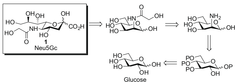
Scheme 1. Retrosynthetic analysis of Neu5Gc synthesis reveals glucose as a suitable starting material. P = protecting group.
