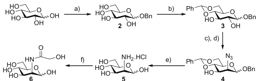
Scheme 2. Synthesis of ManNGc. Reagents and conditions: (a) benzyl alcohol, acetyl chloride, 86%; (b) benzyl-dimethylacetyl, (+)-camphor-10-sulfonic acid, acetonitrile, 84%; (c) pyridine, triflic anhydride, dichloromethane; (d) sodium azide, dimethylformamide, 72% (over two steps); (e) \text{Pd}(\text{OH})_2/\text{C}_{(\text{cat})} , \text{H}_{2(\text{g})} , \text{HCl}_{(\text{aq})} , methanol, 89%; (f) acetoxyacetyl chloride, sodium bicarbonate, water, 94%.
