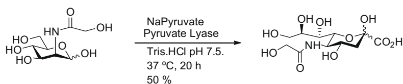
Scheme 3. Enzymatic synthesis of Neu5Gc from ManNGc.
