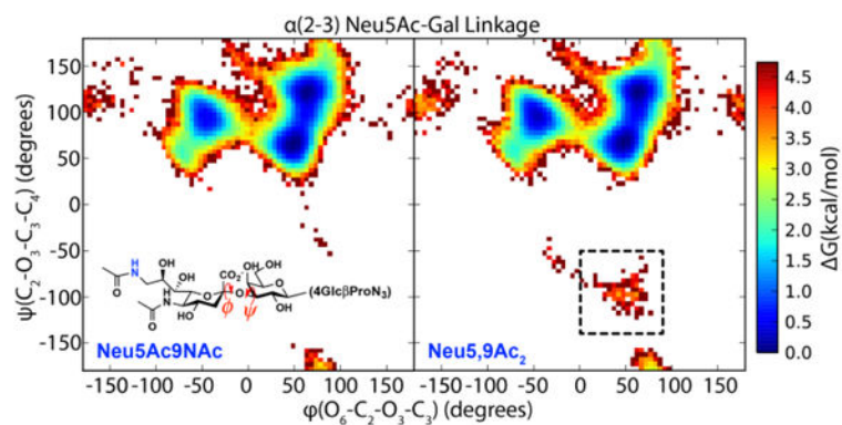
Figure 8. Free energy diagram of glycosidic linkage in solution for Neu5Ac9NAc \alpha 3Gal \beta 4Glc \beta ProN 3 and the corresponding Neu5,9Ac _2 \alpha 3Gal \beta 4Glc \beta ProN 3 . The 9NAc and 9OAc analogs are compared in the left and right panels. The predominant states are almost identical for the two molecules, indicating that the 9NAc and 9OAc sialosides have similar structures in solution. The 9OAc sialoside has a sparsely populated state not seen in 9NAc (dotted box).
