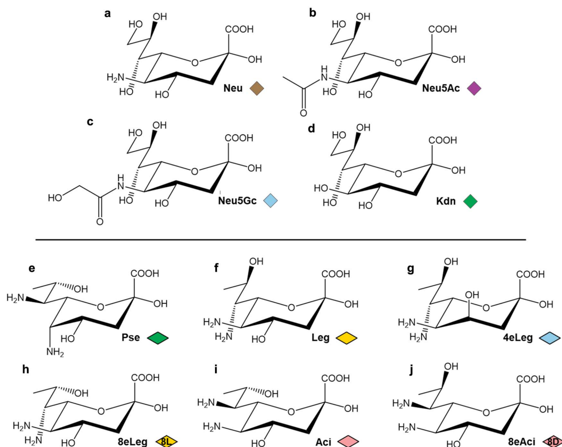
Fig. 1. The non-2-ulonic acids (NulOs). a–d) The 3-deoxy-non-2-ulonic acids (sialic acids): The parent compound in this class is a) neuraminic acid (Neu, 5-amino-3,5-dideoxy-D-glycero-D-galacto-non-2-ulonic acid). The presence of acetamido and hydroxyacetamido substituents at C5 results in b) N -acetylneuraminic acid (Neu5Ac, 5-acetamido-3,5-dideoxy-D-glycero-D-galacto-non-2-ulonic acid), and c) N -glycolylneuraminic acid (Neu5Gc, 3,5-dideoxy-5-hydroxyacetamido-D-glycero-D-galacto-non-2-ulonic acid), respectively. Replacement of the C5 amine with hydroxyl results in d) ketodeoxynononic acid (Kdn, 3-deoxy-D-glycero-D-galacto-non-2-ulonic acid). e–j) The 3,9-dideoxy-non-2-ulonic acids (sialic-acid-like subclass compounds). This family includes six subclasses of compounds: e) pseudaminic acid (Pse, 5,7-diamino-3,5,7,9-tetra-deoxy-L-glycero-L-manno-non-2-ulonic acid), f) legionaminic acid (Leg, 5,7-diamino-3,5,7,9-tetra-deoxy-D-glycero-D-galacto-non-2-ulonic acid), g) 4- epi -legionaminic acid (4eLeg, 5,7-diamino-3,5,7,9-tetra-deoxy-D-glycero-D-talo-non-2-ulonic acid), h) 8- epi -legionaminic acid (8eLeg, 5,7-diamino-3,5,7,9-tetra-deoxy-L-glycero-D-galacto-non-2-ulonic acid), i) acinetaminic acid (Aci, 5,7-diamino-3,5,7,9-tetra-deoxy-L-glycero-L-altra-non-2-ulonic acid), and j) 8- epi -acinetaminic acid (8eAci, 5,7-diamino-3,5,7,9-tetra-deoxy-D-glycero-L-altra-non-2-ulonic acid). The ^2C_5 chair conformations of Neu, Neu5Ac, Neu5Gc, Kdn, Leg, 4eLeg, and 8eLeg are presented in the \alpha -anomeric configuration and the ^2C_5 chair conformations of Pse, Aci, and 8eAci are in the \beta -anomeric configuration. Note that in all structures shown here, the COOH group at C2 has an axial orientation. All SNFG figures in this report were rendered using DrawGlycan-SNFG (Cheng et al. 2017).
